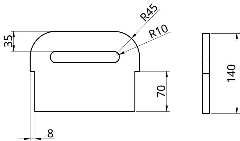
HANDLE
